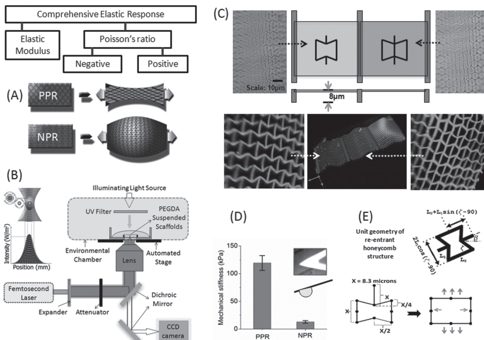
Figure 1. A) The elastic property of a biomaterial can be comprehensively expressed by the elastic modulus and the Poisson's ratio. Schematic shows a PPR material contracting transversally when axially stretched, while a NPR material expanding in both the axial and transverse directions. B) Schematic of the two-photon absorption process and the femtosecond laser fabrication set-up. C) Optical and confocal images of NPR and PPR suspended web structures with side supports using PEGDA biomaterial. D) AFM measurements using a 20 \mu\text{m} bead measures the effective stiffness of NPR and PPR web structures in the z-direction. E) Re-entrant honeycomb configuration was adopted as the unit cell geometry for the NPR web, while an additional strut modification to the NPR structure served as the positive control. Schematic shows biaxial expansion of the NPR structure upon axial strains (arrows)
