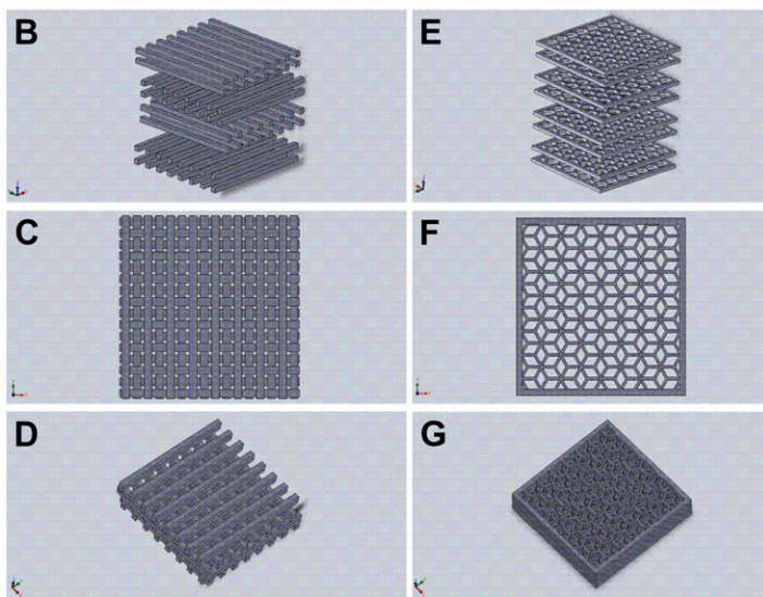
Schematic diagram of woodpile scaffold (B–D)
