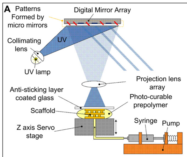
Schematic diagram of Digital Mirror Device (DMD) system
