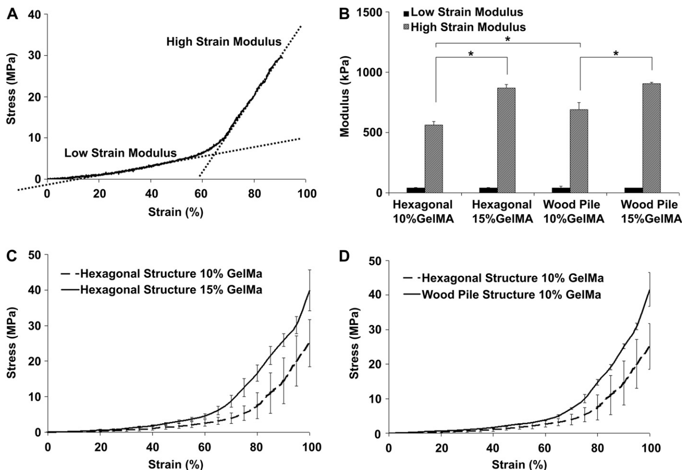
Fig. 3. Mechanical properties of PSL-fabricated scaffolds having hexagonal or log pile structures and fabricated using various GelMA percentages. A characteristic stress-strain curve displaying low-strain and high-strain compressive moduli was obtained for every sample tested (A). Results showed that high-strain modulus was significantly increased for both hexagonal and woodpile structures when the percentage of GelMA was increased from 10%–15%, whereas no significant difference was seen for the low-strain modulus in any conditions (B). Compressive testing results indicate that prepolymer concentration (C) and engineered structures (D) can be used to tailor the mechanical properties of the GelMA scaffolds. * indicates statistical significance ( p < 0.05 ).
